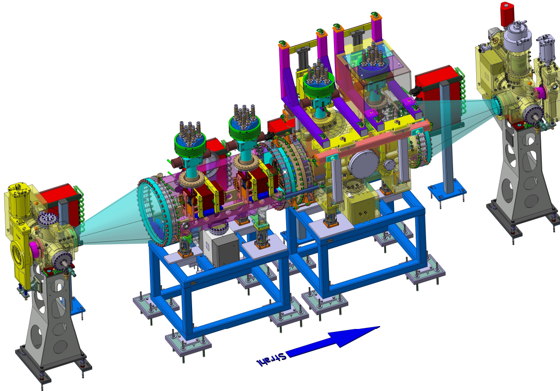
Figure 2: Design of the HESR injection kicker system. The system consist of four magnets inside of two vacuum tanks. The tanks are delivered separately and connected together at place using special bellow. Each magnet is connected to semiconductor based pulser using six coaxial cables which are joint together in one HV feed-trough at the top of the vacuum tank. A lifting system is designed to prevent damages of the ceramic feed-trough due to the external forces at the cable and disconnect the systems from the pulsers for the time of the bake-out process. Special conical tubes are designed to smoothen injection section impedance for the particle beam. In addition to the turbo and ion pumps at each vacuum tank, there are also standard HESR pump systems installed at both sides of the kicker section.
